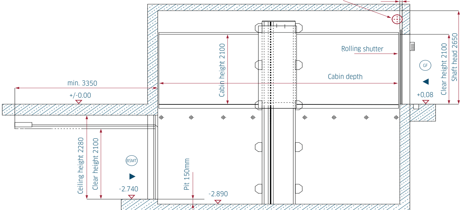
Rolling shutter in shaft head Niche 52mm
