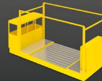
10 TRANSFER VEHICLE The transfer vehicle is used for transporting cargo horizontally on a single level. The individual loading units are moved on and off the racking by interconnecting the integrated roller conveyor with external roller decks. As well as transporting ULDs which can take up the entire surface of the roller deck, it is possible to transfer two containers simultaneously.
